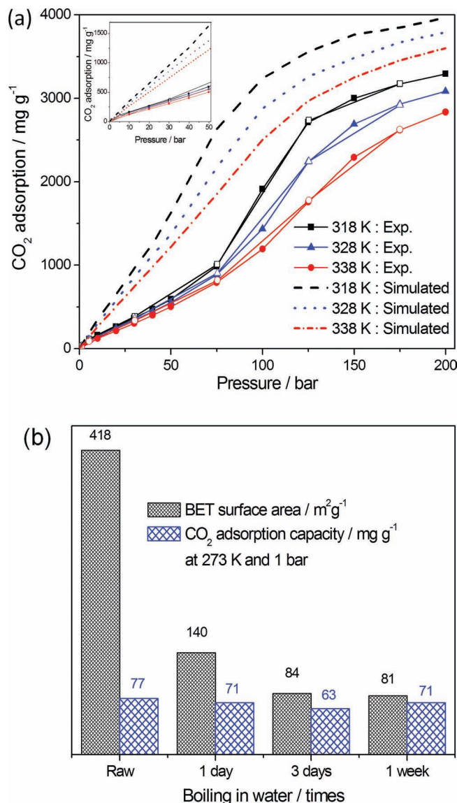
Figure 3. a) High pressure CO 2 adsorptions for COP–3 measure at 318, 328, and 338 K up to 200 bar. CO 2 adsorption (filled symbols)–desorption (open symbols). Theoretical simulated isotherms (dashed lines) show similar shapes and temperature dependency as experimental isotherms. Inset: 0–50 bar region was magnified for better display. b) Effect of boiling in H 2 O on BET surface area and low pressure CO 2 adsorption capacities.
