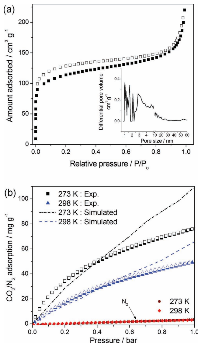
Figure 2. a) Ar adsorption–desorption isotherm measured at 87 K (inset: pore size vs differential pore volume); b) Low pressure CO 2 and N 2 adsorptions for COP–3 at 273 and 298 K up to 1 bar. Adsorption (filled symbols), desorption (open symbols). Theoretical simulation (dashed lines) shows a near fit to the experimental values below 0.5 bar.
